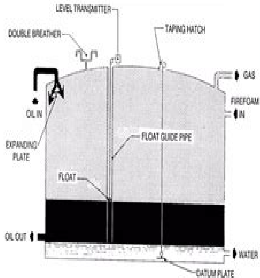
FIXED ROOF TANK
