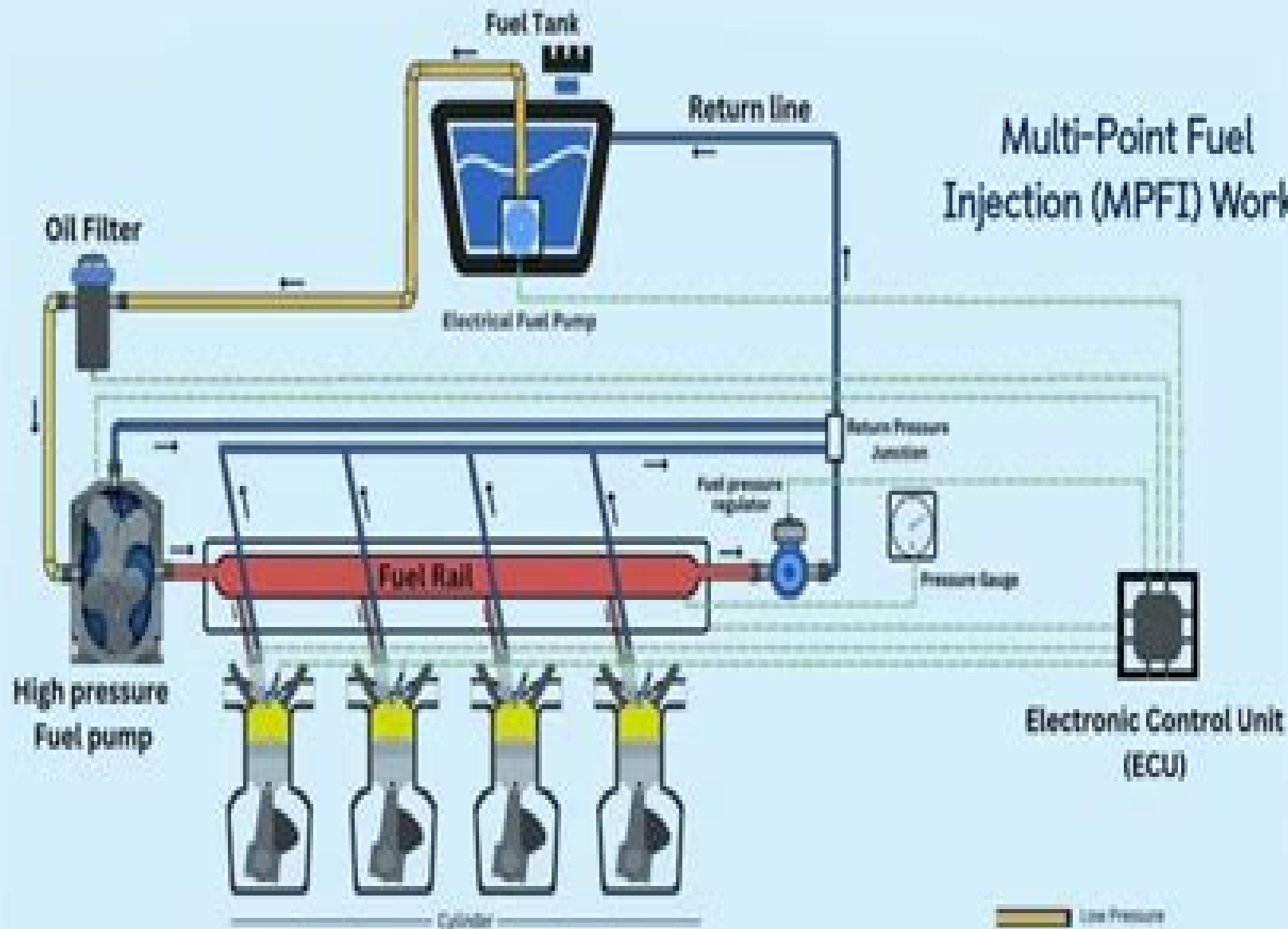
Multi Point Fuel injection system
