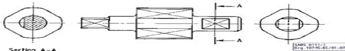
Figure 29 — Square on a shaft and flat face on a cylinder
