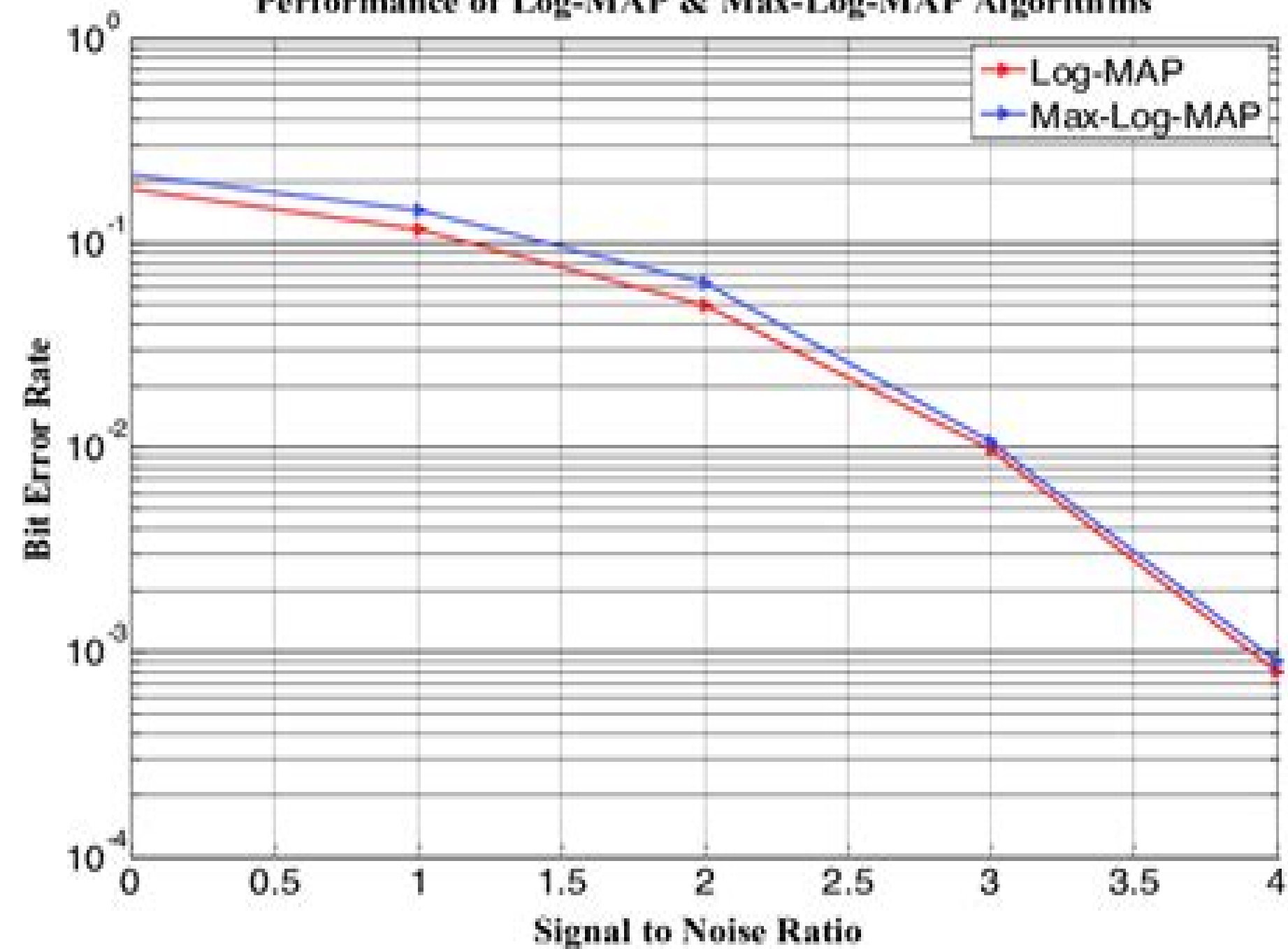
Performance of Log-MAP & Max-Log-MAP Algorithms
