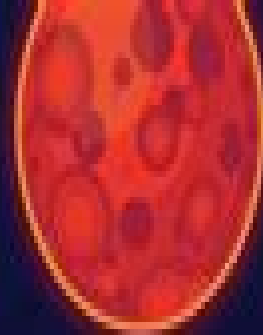
PROXIMA CENTAURI
